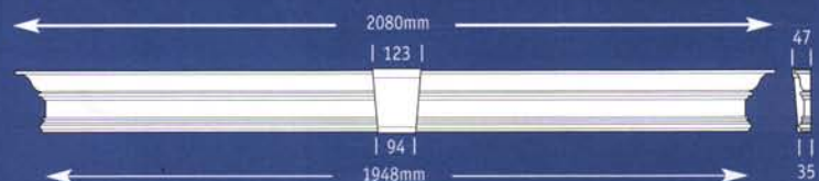
A506 Lime Double door pediment-3 pc Overall depth can be reduced
